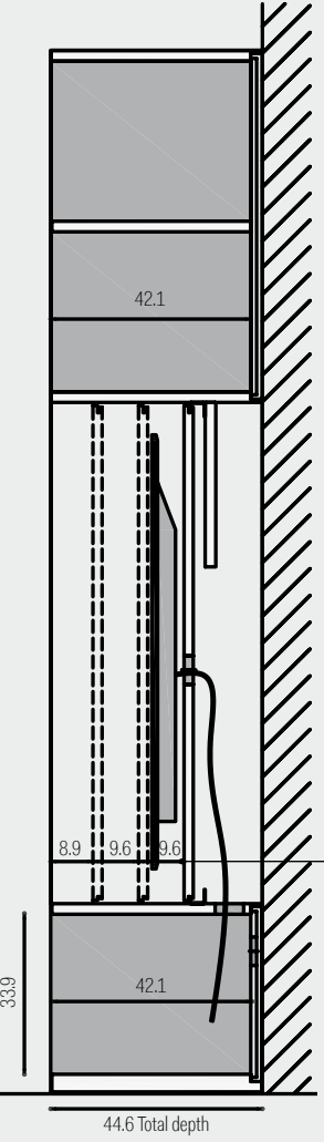
TV compartment Total depth 44.6 cm Open or for sliding door Side view
