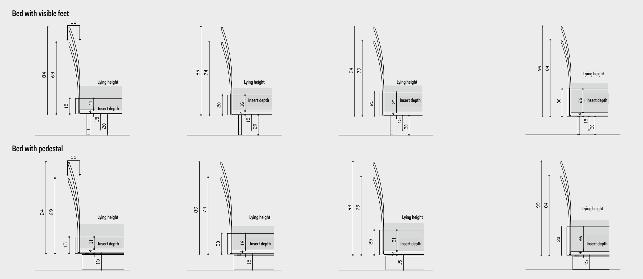
Bed with feet or pedestal with a curved headboard – dimensions in cm, A = inner dimensions
