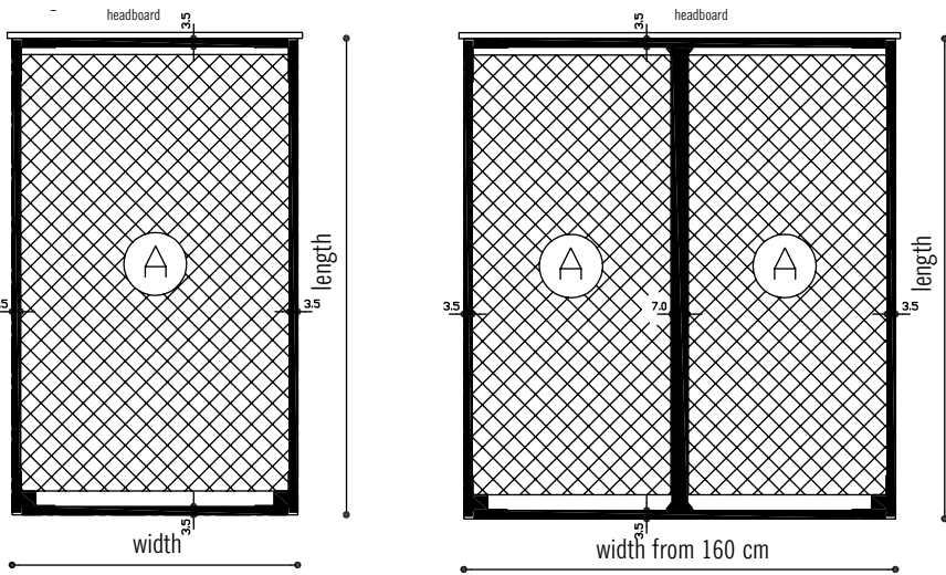
Bed with feet or pedestal with a straight headboard – dimensions in cm, A = inner dimensions
