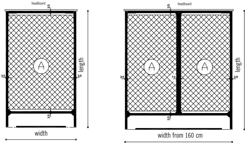
Floating bed with straight headboard – dimensions cm, A = inner dimensions
