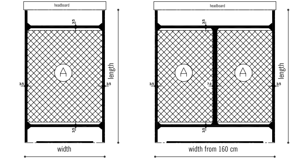
Floating bed with a curved headboard – dimensions cm, A = inner dimensions
