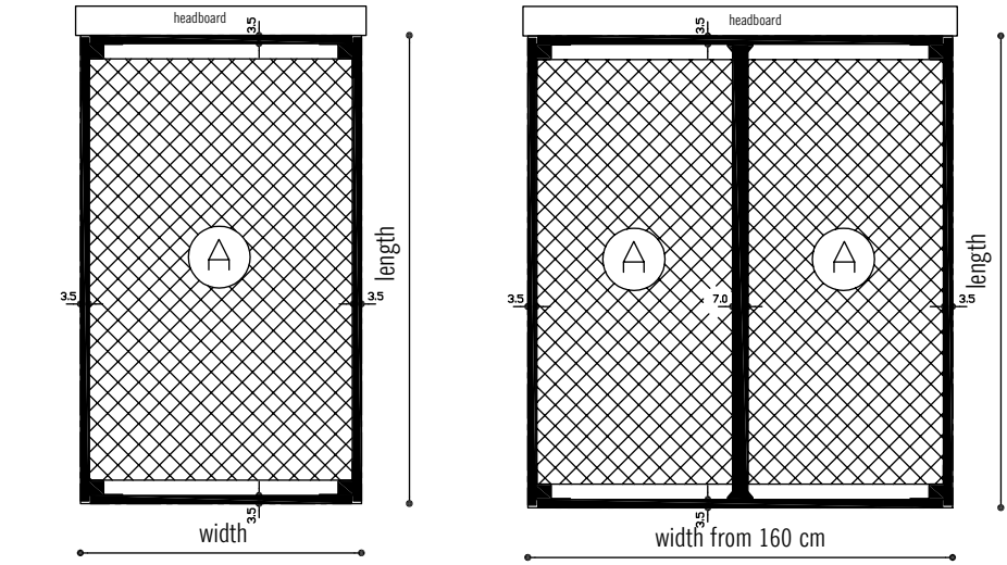
Bed with feet or pedestal with a curved headboard – dimensions in cm, A = inner dimensions
